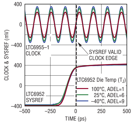
7.25GHz JESD204B/C CLK to SYSREF Alignment Calibration Over Temperature
