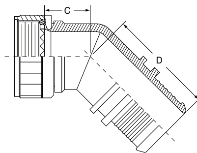
45° ENTRY ROTATABLE COUPLING 2M440MK135
