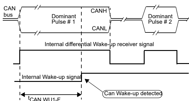
Figure 35. Single dominant pulse wake-up
