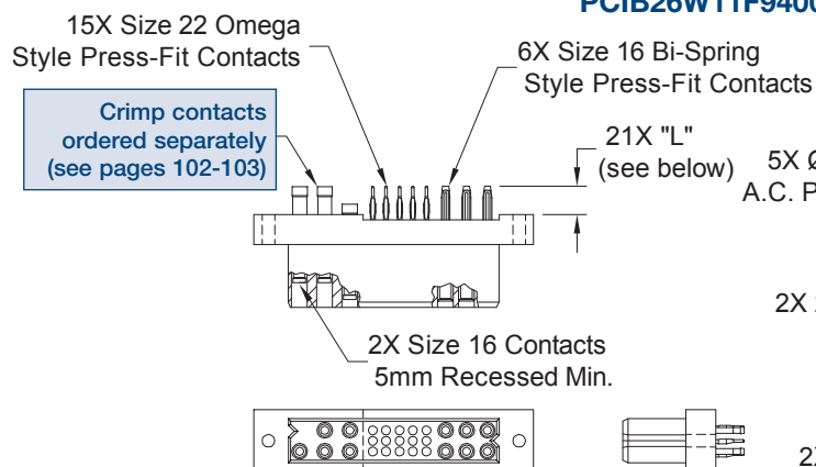
CONNECTOR DIMENSIONS
