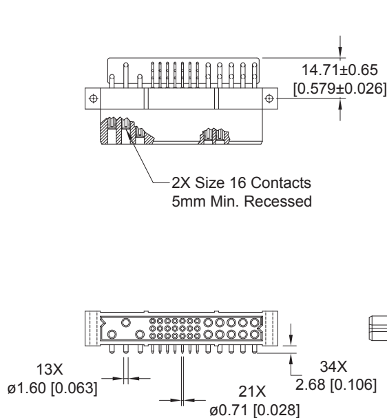
CONNECTOR DIMENSIONS
