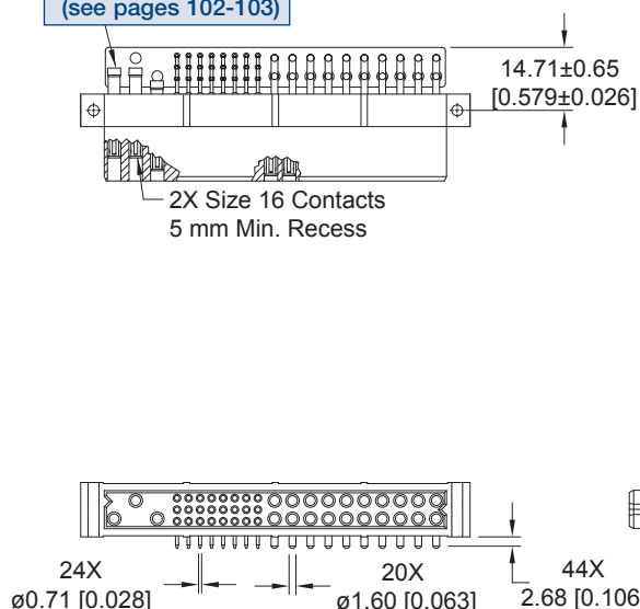
CONNECTOR DIMENSIONS
