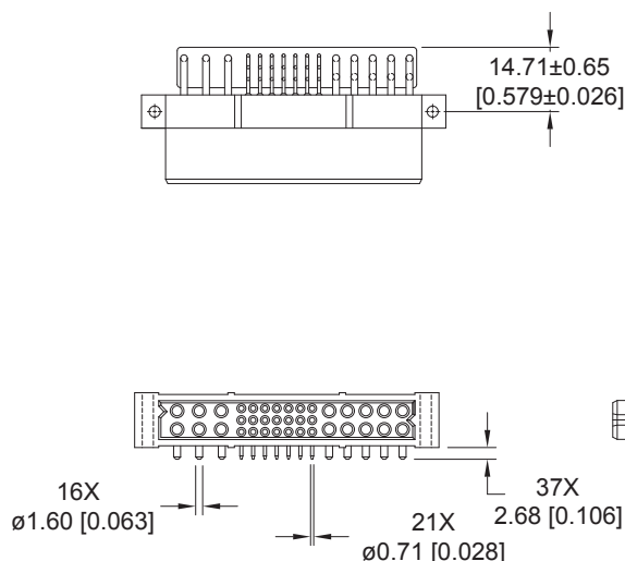
CONNECTOR DIMENSIONS
