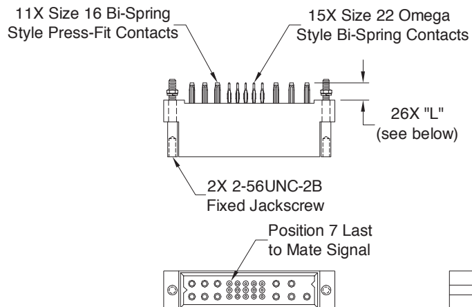
CONNECTOR DIMENSIONS
