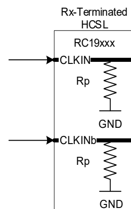
Figure 17. Receiver Termination
