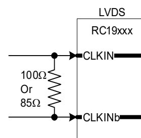
Figure 15. LVDS Input Levels
