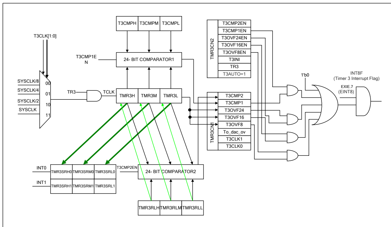
TMR3CN1 (A100h) Timer 3 Control Register One R/W 00000000
