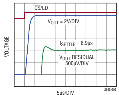
Settling 10V Step
