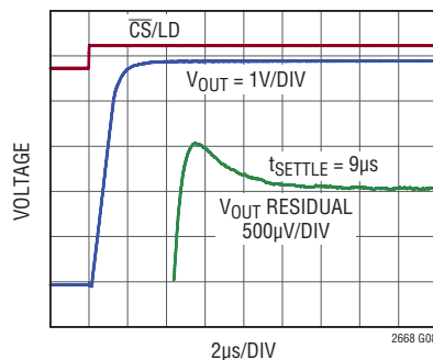
Settling 5V Step
