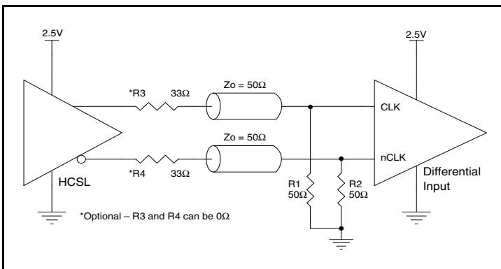
Figure 10C. CLKx/nCLKx Input Driven by a 2.5V HCSSL Driver
