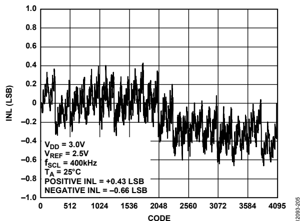
Figure 5. INL vs. Code
