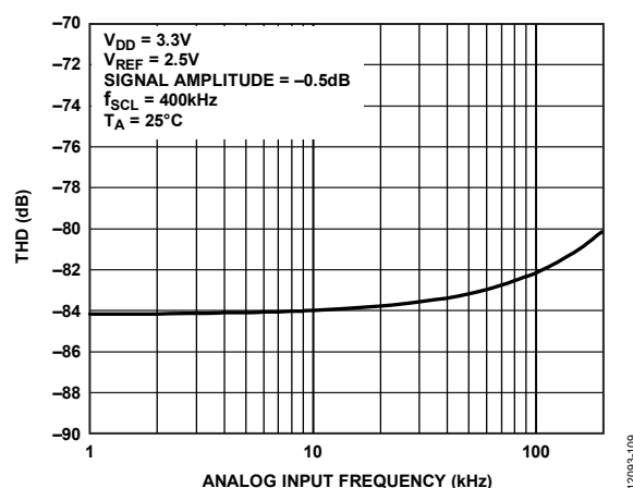
Figure 15. THD vs. Analog Input Frequency
