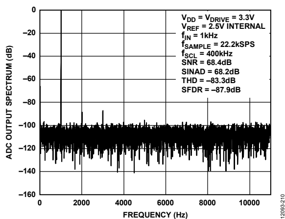
Figure 12. 10 kHz FFT, V_{DD} = 3.0\text{ V} , V_{REF} = 2.5\text{ V} Internal
