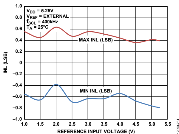
Figure 6. Minimum/Maximum INL vs. External Reference Input Voltage
