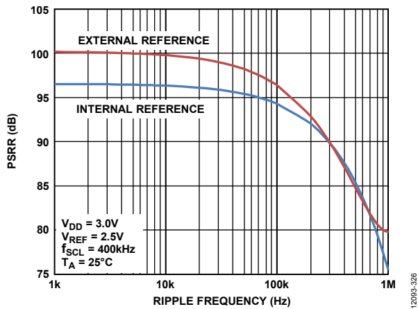
Figure 25. PSRR vs. Ripple Frequency
