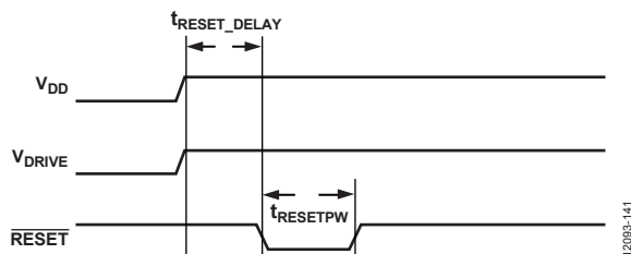
Figure 35. RESET Pin Power Up Timing
