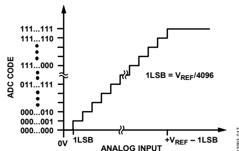
Figure 34. Transfer Characteristic
