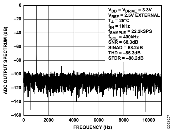
Figure 11. 10 kHz FFT, V_{DD} = 3.0\text{ V} , V_{REF} = 2.5\text{ V} External
