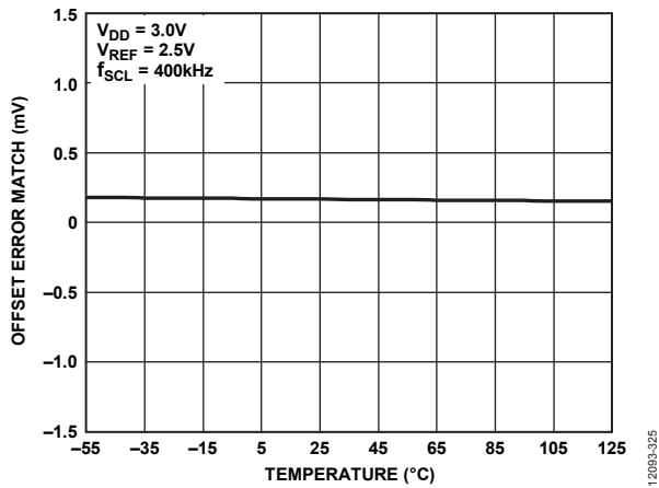
Figure 24. Offset Error Match vs. Temperature
