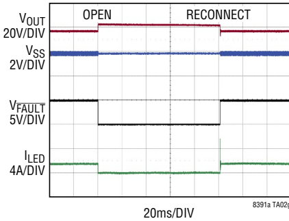
OPEN LED Protection: Keep-Running Mode ( R_{SS} = 100k )
