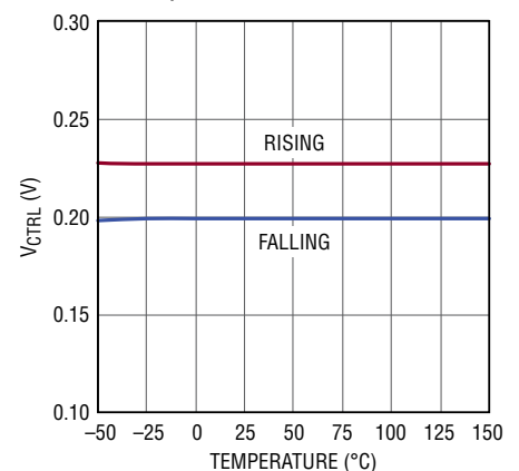
CTRL1/CTRL2 Dim-Off Threshold
