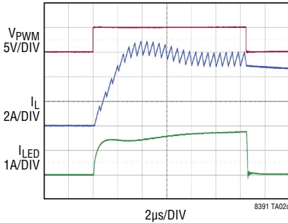
100Hz 800:1 External PWM Dimming ( V_{IN} = 8V )
