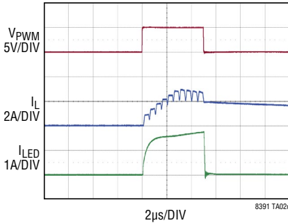
100Hz 2000:1 External PWM Dimming ( V_{IN} = 18V )
