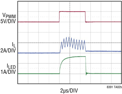
100Hz 2000:1 External PWM Dimming ( V_{IN} = 32V )
