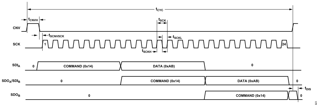
Figure 54. Register Write Timing Diagram, Daisy-Chain Mode
