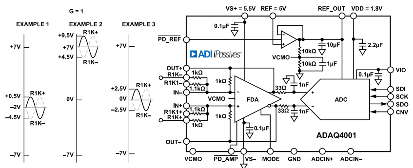
Figure 47. Differential Configuration with G = 1
