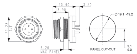
PANEL CUT-OUT
