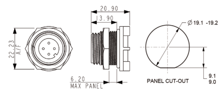
PANEL CUT-OUT
