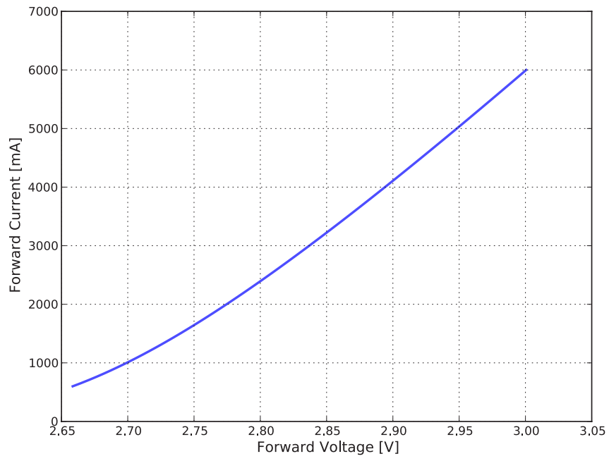
Figure 5c. Typical forward current vs. forward voltage for L1MX-xxxx03Vxxxxx0 at T j =85°C.
