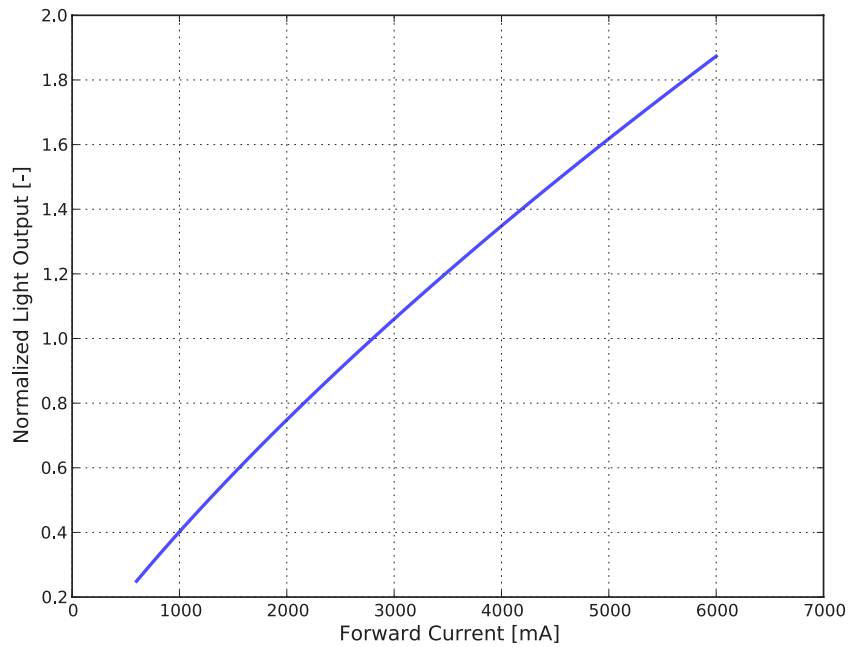
Figure 4c. Typical normalized light output vs. forward current for L1MX-xxxx03Vxxxxx0 at T_j=85^\circ\text{C} .
