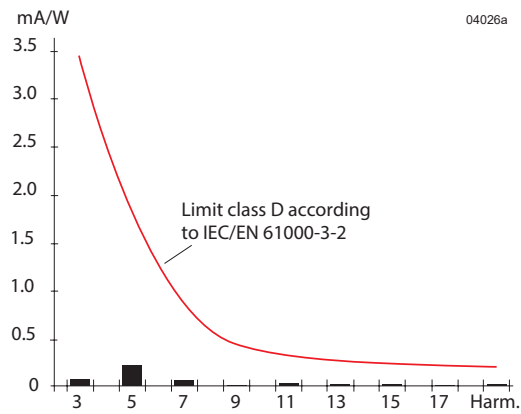
Fig. 4 Harmonic distortion at input LT1740-7Z, V_i = V_{inom} , I_o = I_{o nom}
