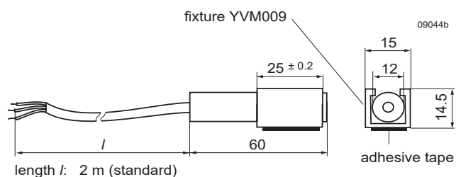
Fig. 61 Mechanical dimensions (in mm)
