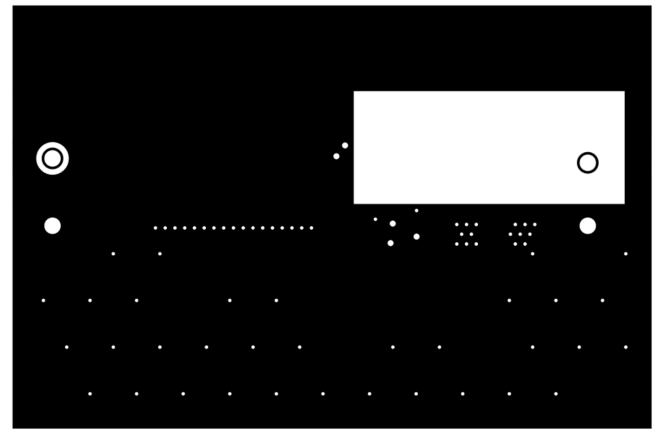
Figure 8. Bottom Layer
