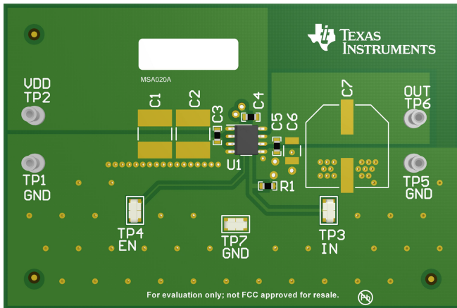
Figure 3. Top Assembly
