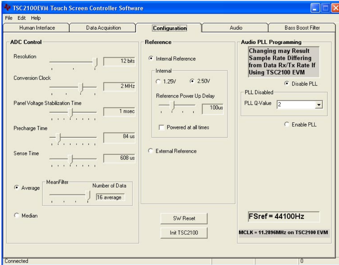
Figure 3–6. Configuration Screen
