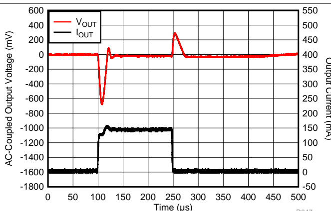
Output current slew rate = 150 mA/ \mu\text{s}
