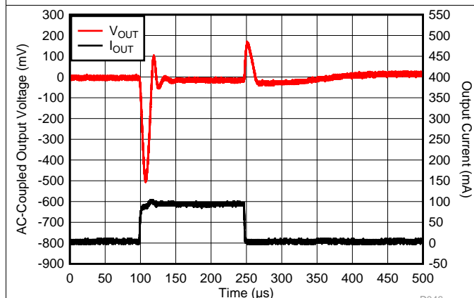
Output current slew rate = 100 mA/ \mu\text{s}
