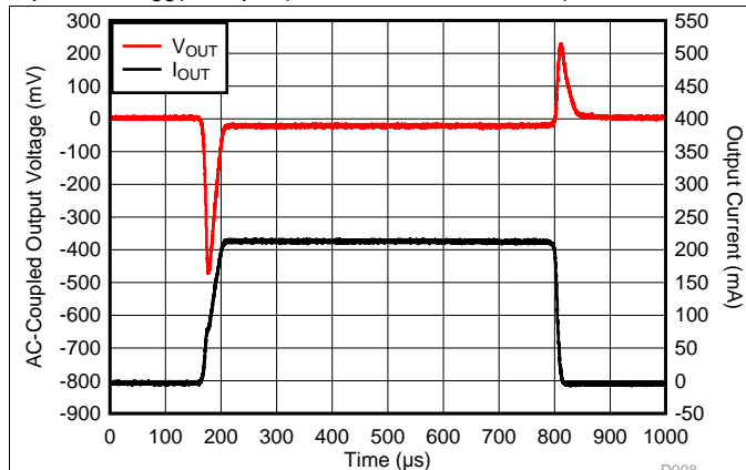
Output current slew rate = 6.6 mA/ \mu\text{s}
