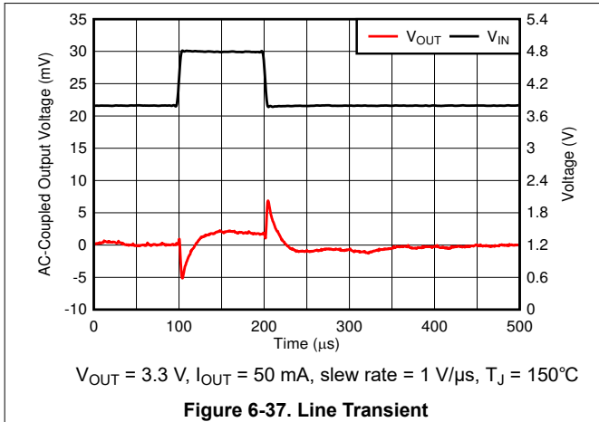
Figure 6-37. Line Transient
