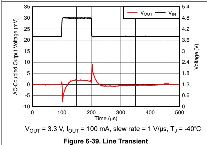
Figure 6-39. Line Transient
