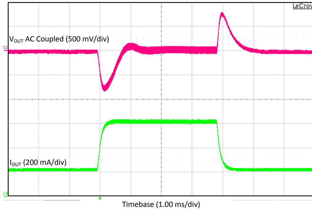
Figure 4. TPS55340EVM-017 V_{IN} = 5\text{-V} Transient Response
