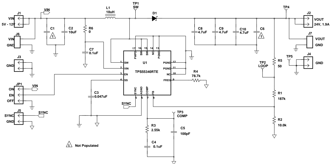
Figure 22. TPS55340EVM-017 Schematic
