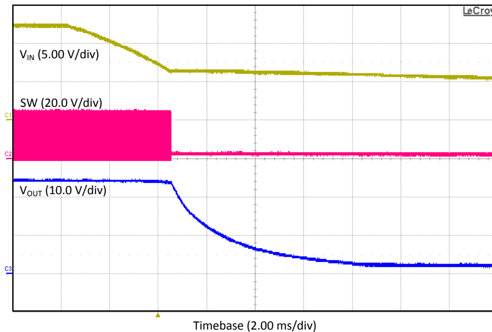
Figure 16. TPS55340EVM-017 Power Down With V_{IN}
