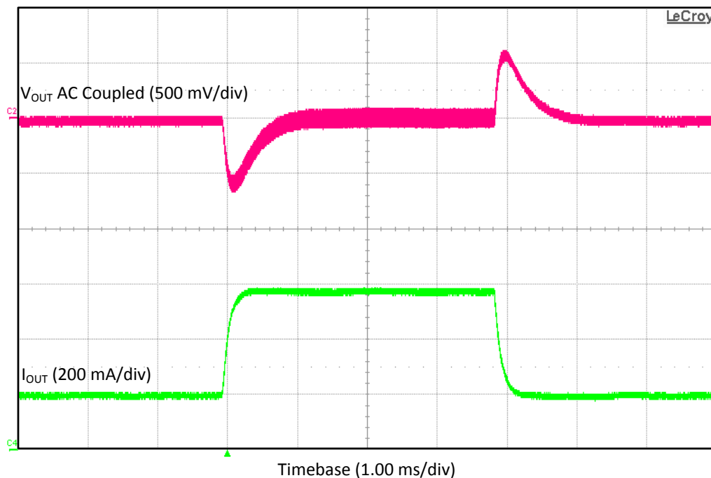
Figure 5. TPS55340EVM-017 V_{IN} = 12\text{-V} Transient Response
