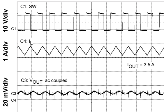
Time = 2 μs/div Figure 10. Output Voltage Ripple CCM
