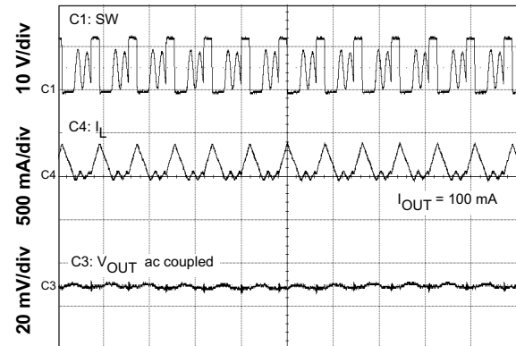
Time = 2 μs/div Figure 11. Output Voltage Ripple DCM
