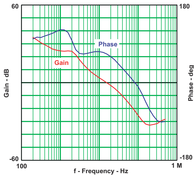
Figure 2-9. TPS5430 Loop Response
