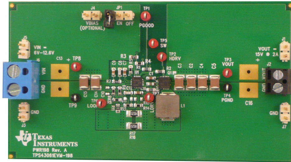
Figure 1. TPS43061EVM-198 EVM Board
